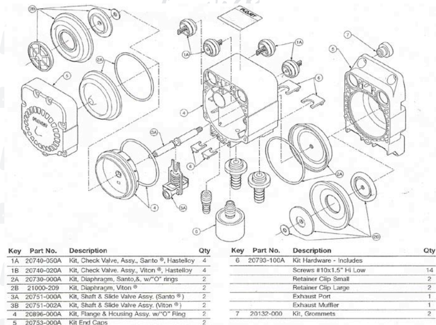
Model G57 series exploded view
