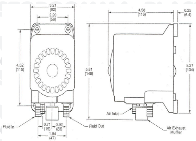
Dimensional drawing
